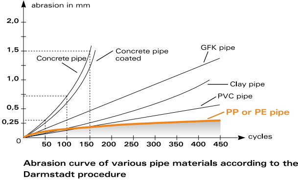
Abrasion curve of various pipe materials according to the Darmstadt procedure
