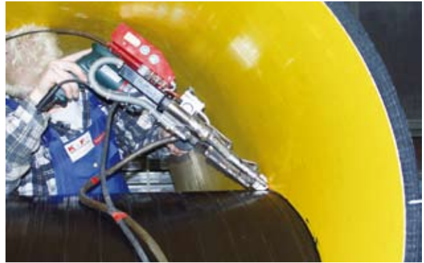
Fabricating of a fitting
