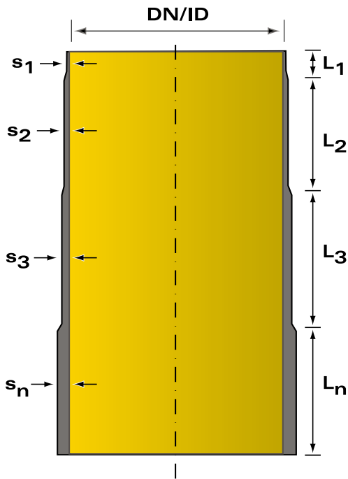
Sketch of a stepped vertical storage tank s_1 = wall thickness of the step i L_1 = length of the step i
