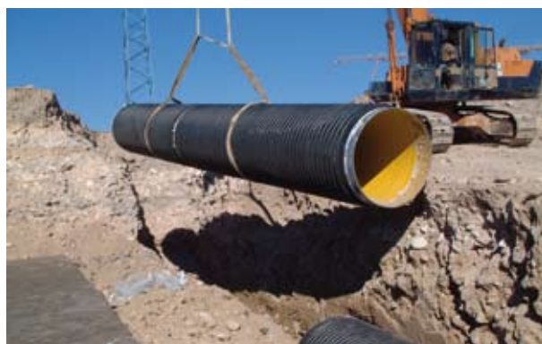
Installation of two pre-jointed pipes DN 1600mm
