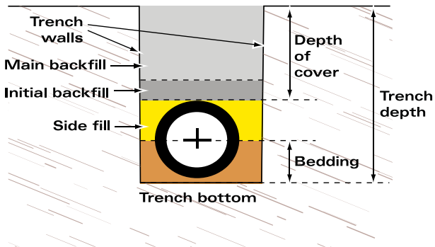
Installation of a Krah pipe acc. to EN 1610
